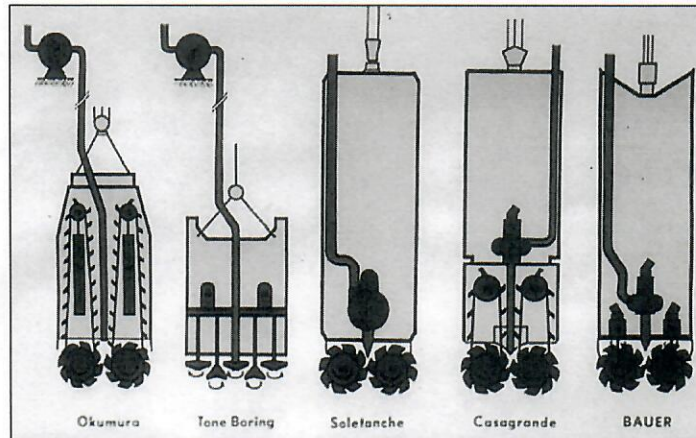
Development of Trench Cutters
