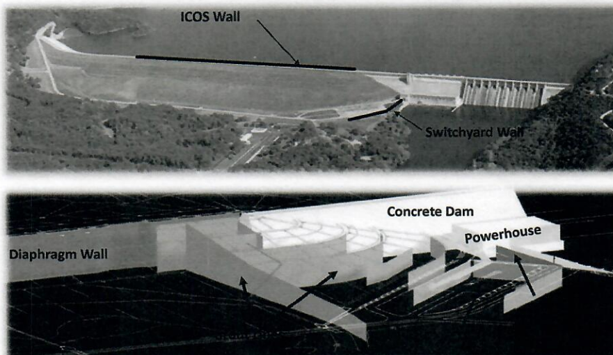
First Solution – Cutoff Wall and Extensive Grouting Campaigns
