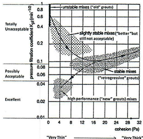
Figure 2. Historical path of development from unstable mixes to contemporary balanced multi-component mixes (modified after De Paoli et al., 1992).
